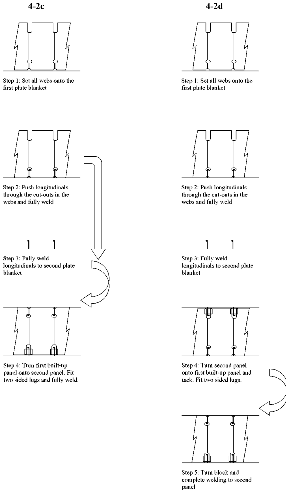
Fig. 3.37. Block assembly methods 4-2c and 4-2d [2], [30]
