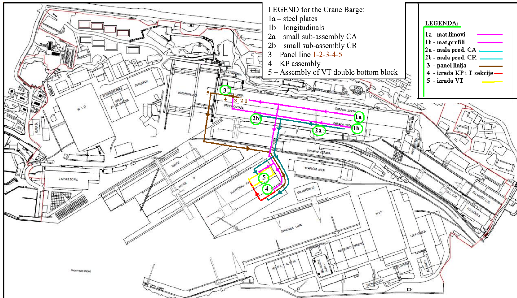
Fig. 4.30. Flow of material during the assembly of the double bottom block for the Crane barge in 3.Maj shipyard [30]
