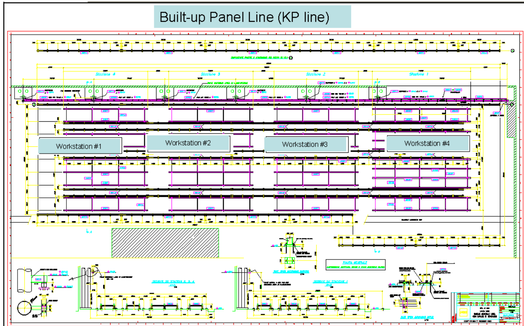
Fig. A7. Built-up panel (KP) line with workstations [30]
