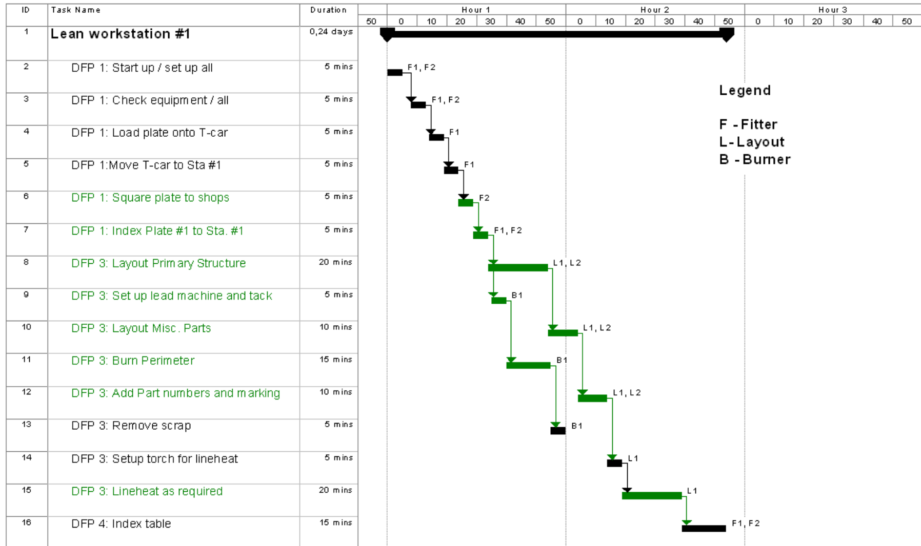
Fig. 5.14. Lean Workstation 1 Gantt chart
