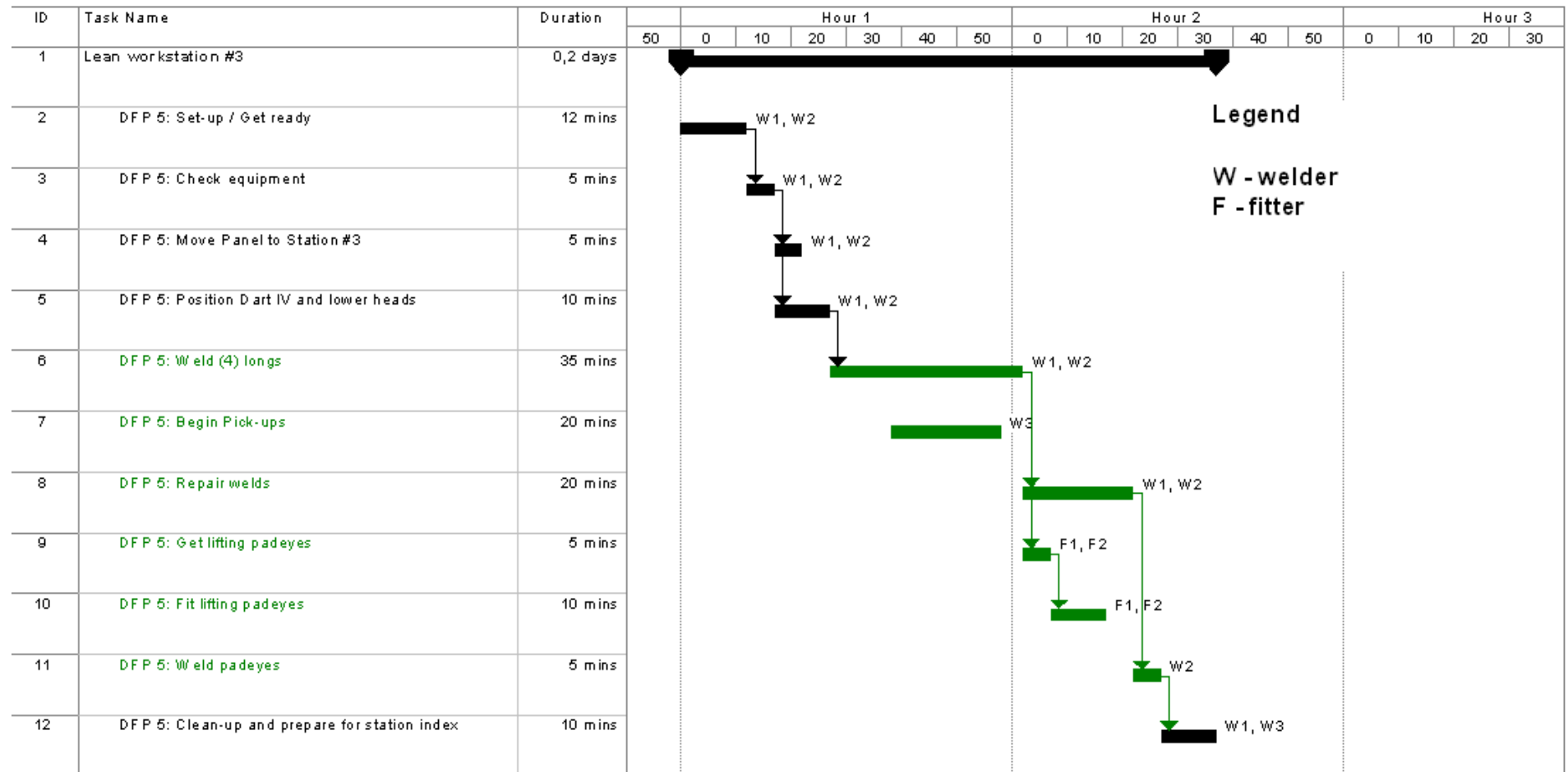
Fig. 5.16. Lean Workstation 3 Gantt chart
