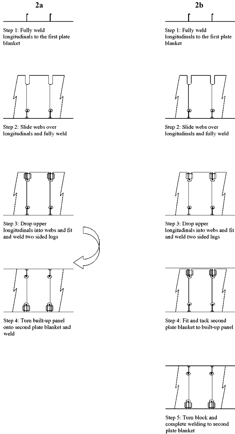
Fig. 3.16. Block assembly methods 2a and 2b [2], [30]
