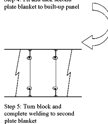
Fig. 3.49. Block assembly method 5-2g [2], [30]
