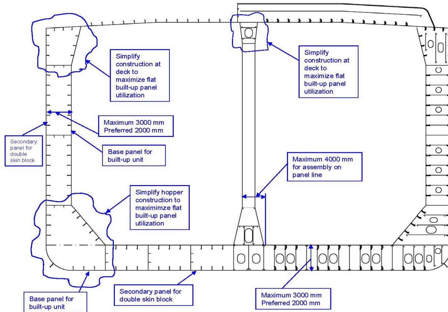
Fig. 7.1. Generic midship section of a chemical tanker with constraints for present production program [2], [30], [47]
