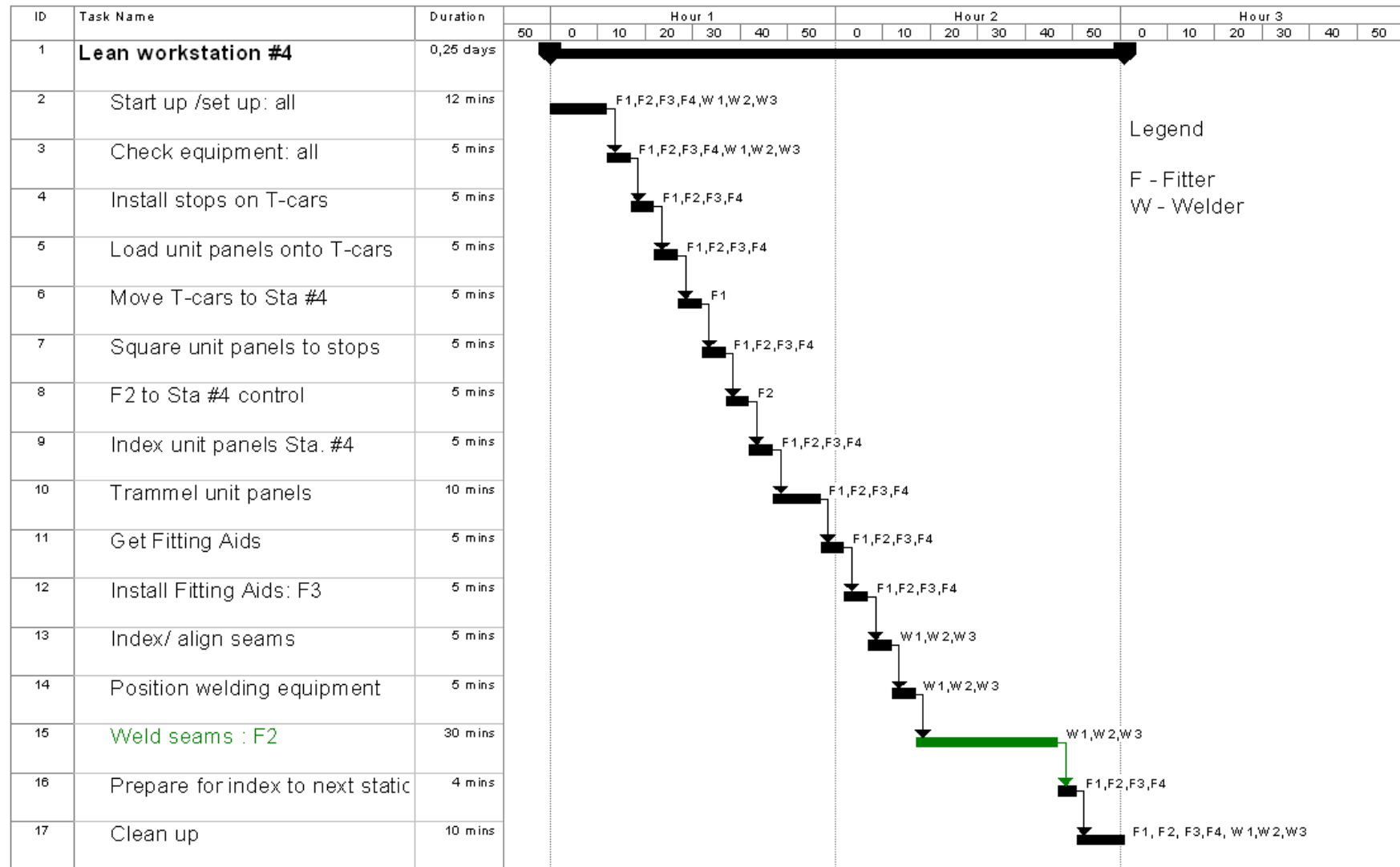
Fig. 5.17. Lean Workstation 4 Gantt chart
