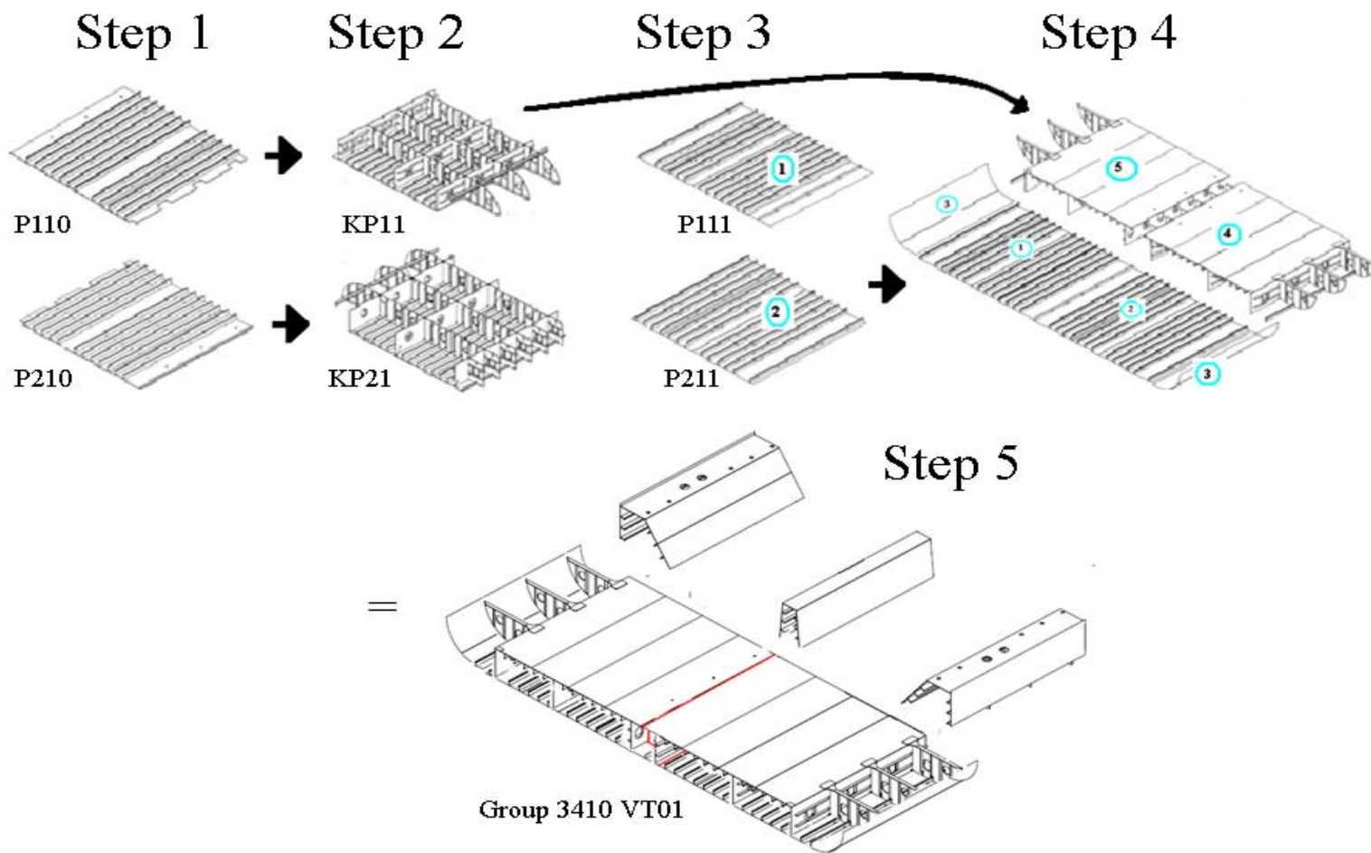
Fig. 4.9. General plan for assembling the double bottom 3410 VT01 of the Chemical tanker with work phases [30]
