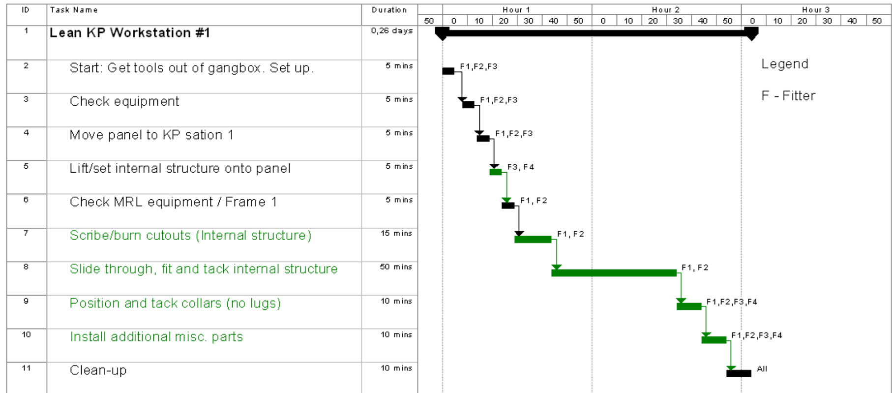
Fig. 5.18. Lean KP Workstation 1 Gantt chart
