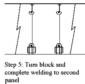
Fig. 3.47. Block assembly methods 5-2c and 5-2d [2], [30]
