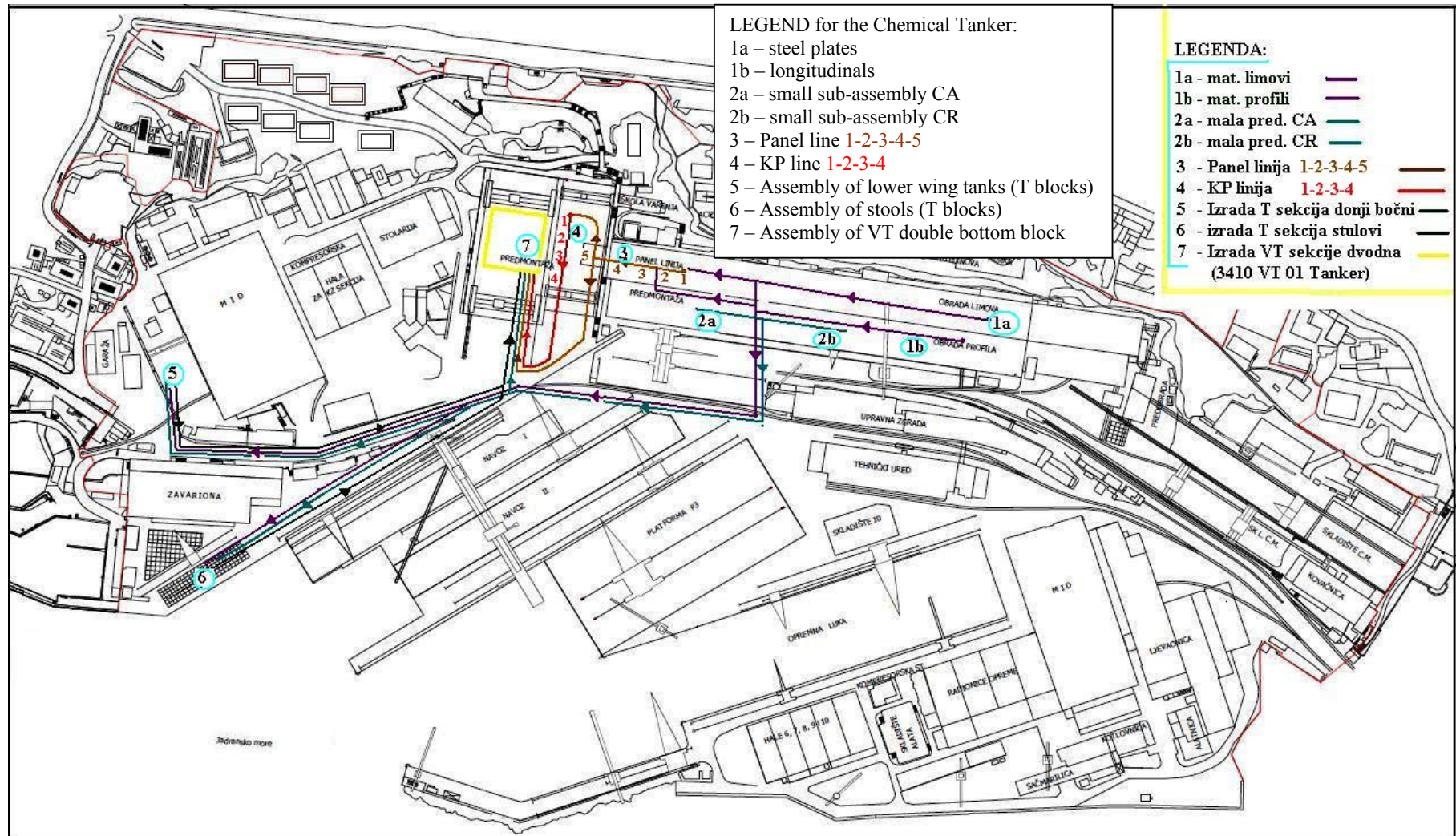
Fig. 4.28. Flow of material during the assembly of the double bottom block for the Chemical tanker in 3.Maj shipyard [30]
