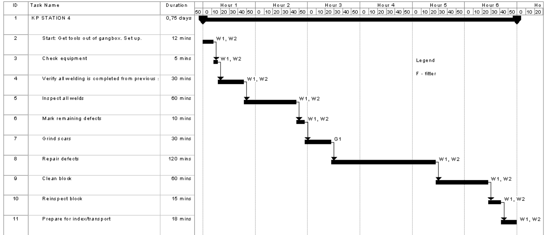
Fig. 4.27. KP Workstation 4 Gantt chart [2], [30]
