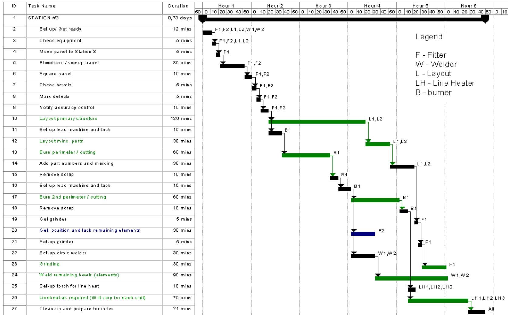
Fig. 4.21. Workstation 3 Gantt chart [2], [30]
