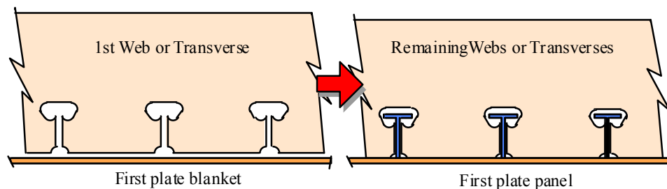
Fig. 3.5. Principal block assembly method 3-2 [2]
