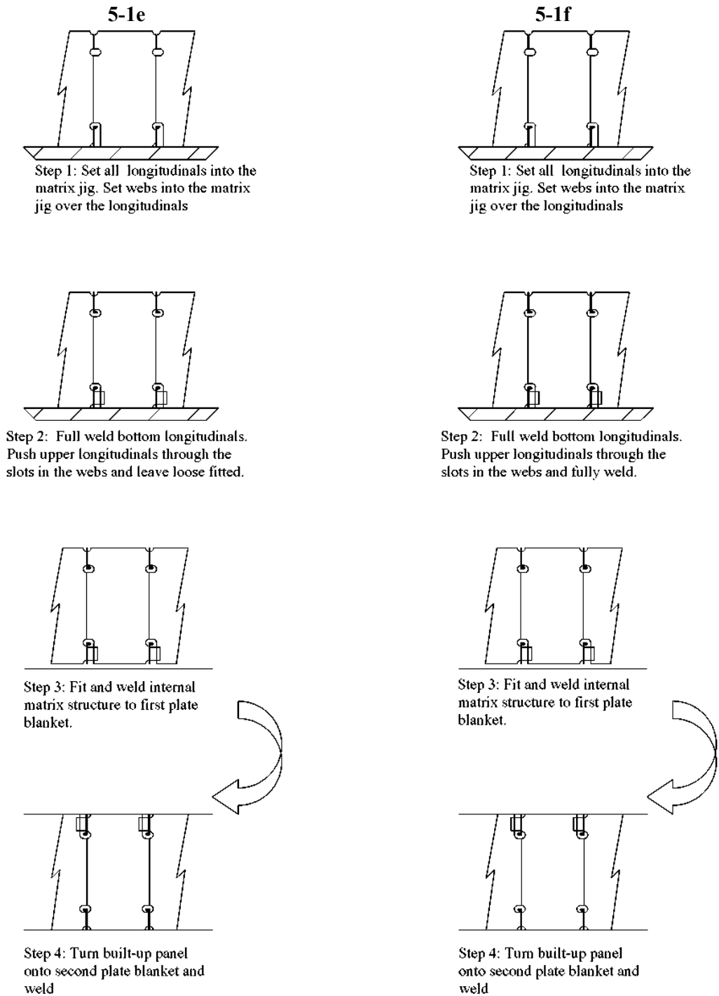
Fig. 3.43. Block assembly methods 5-1e and 5-1f [2], [30]
