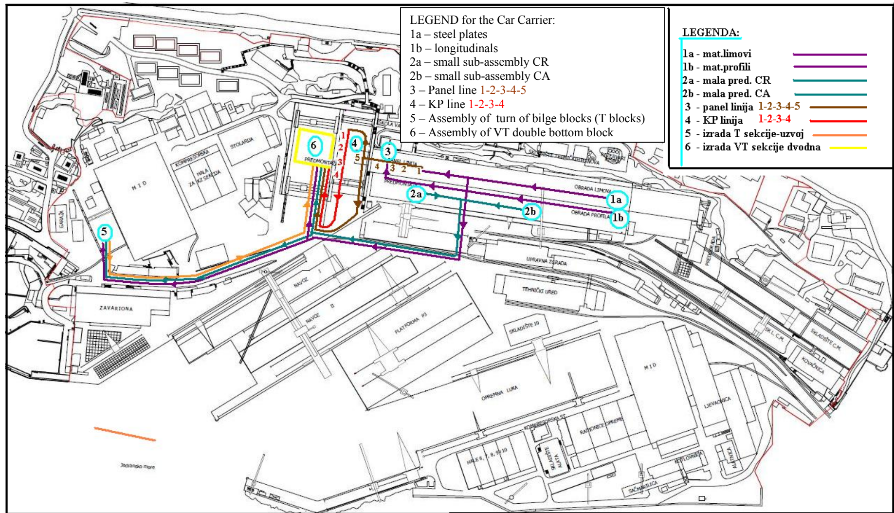
Fig. 4.29. Flow of material during the assembly of the double bottom block for the Car carrier in 3.Maj shipyard [30]
