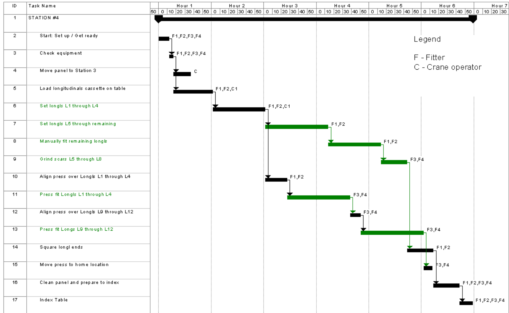
Fig. 4.22. Workstation 4 Gantt chart [2], [30]
