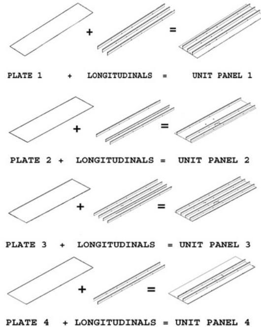
Fig. 5.2. Assembly sequence on the Lean unit-panel assembly line
